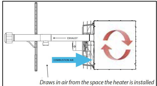
Power Vented Unit Heater
