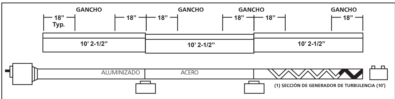
FIGURE 2D: Heatstar AG Model HSAG-100 Assembly Overview
