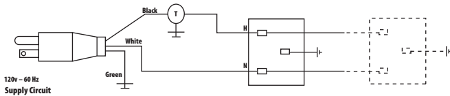
FIGURE 14: Line Voltage Thermostat Wiring Burners (Maximum - 2 per Thermostat)
