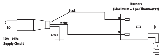
FIGURE 15: Low Voltage Thermostat Wiring
