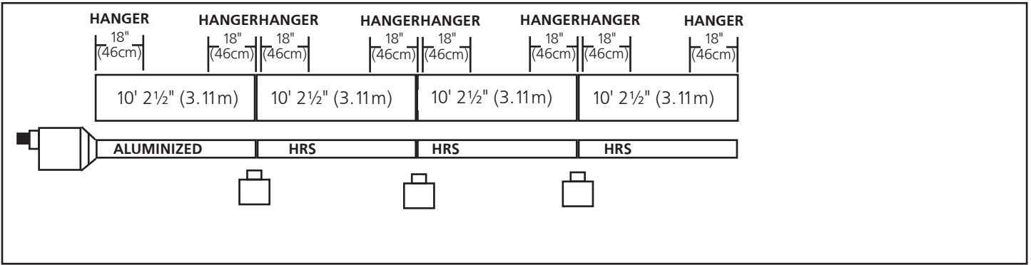
FIGURE 2F: Heatstar AG Model HSAG-125, HSAG-150, HSAG-175
