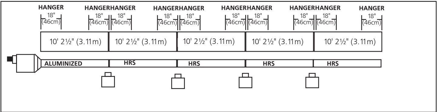
FIGURE 2G: Heatstar AG Model HSAG-150, HSAG-175
