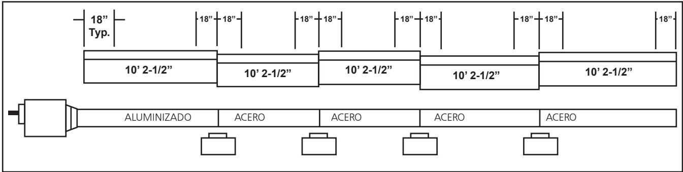
FIGURE 2G: Heatstar AG Model HSAG-150, HSAG-175
