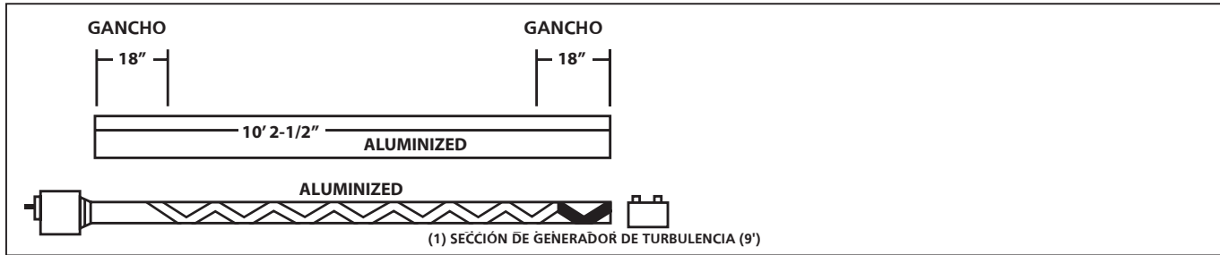
FIGURE 2B: Heatstar AG Model HSAG-60, HSAG-80, Assembly Overview
