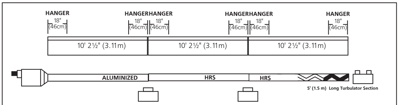
FIGURE 2D: Heatstar AG Model HSAG-100 Assembly Overview
