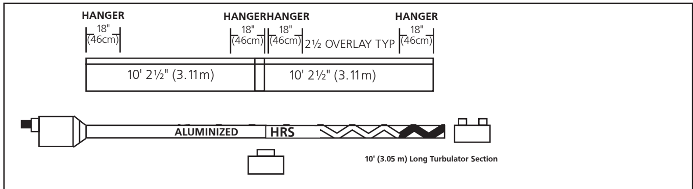
FIGURE 2C: Heatstar AG Model HSAG-80, Assembly Overview
