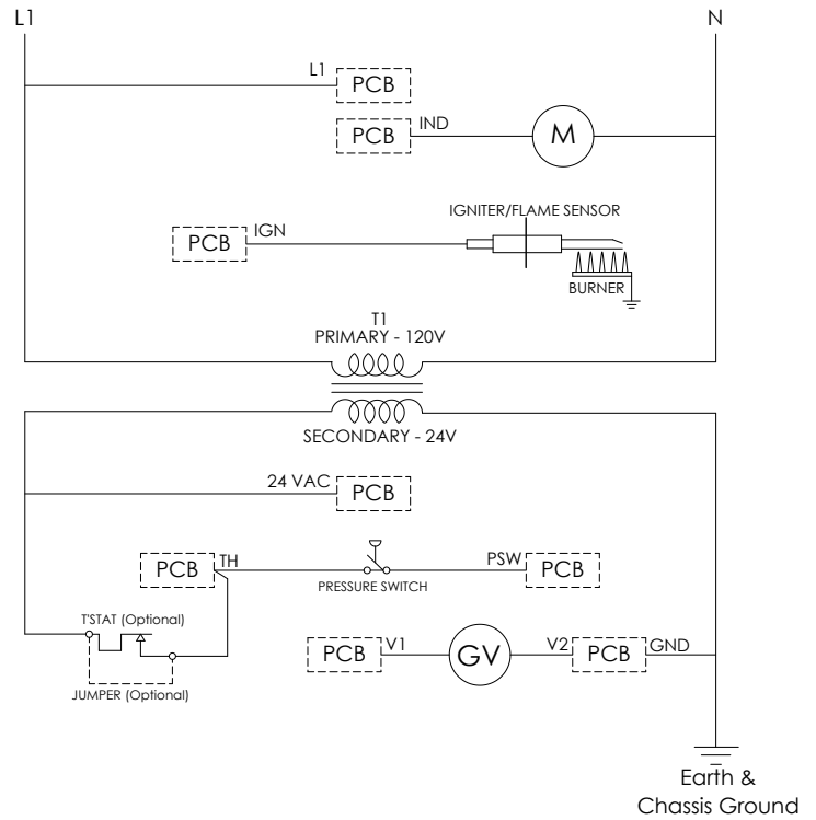
FIGURE 17: Heatstar AG Burner Internal Wiring Ladder Diagram
